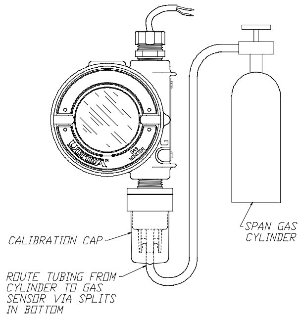
Figure 2-7. Span Gas Connection (Ultima unit shown)
