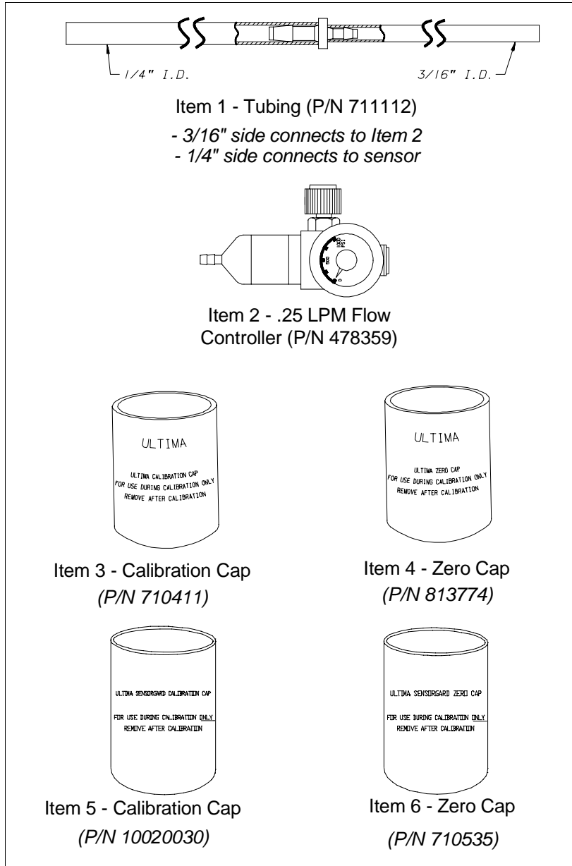
Figure 2-2. Calibration Kit 41 Contents (Your Kit may also include one or two gas cylinders)
